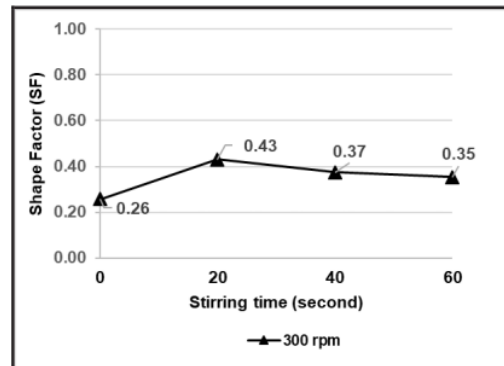
Fig. 3. Effect of stirring time on the shape factor of the primary particles.
