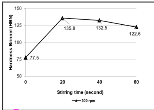
Fig. 4. Effect of stirring time on the hardness.
