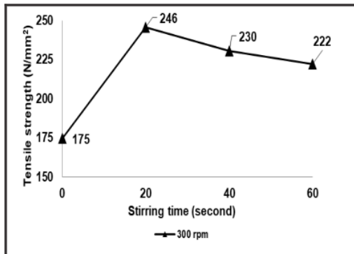
Fig. 5. Effect of stirring time on the tensile strength.
