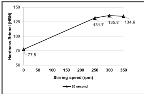
Fig. 9. Effect of stirring speed on the hardness.
